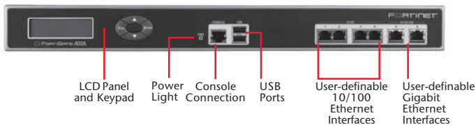
FortiGate-400A
