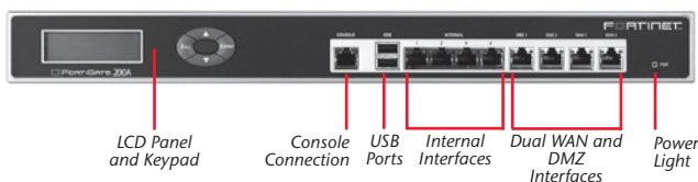
FortiGate-200A
